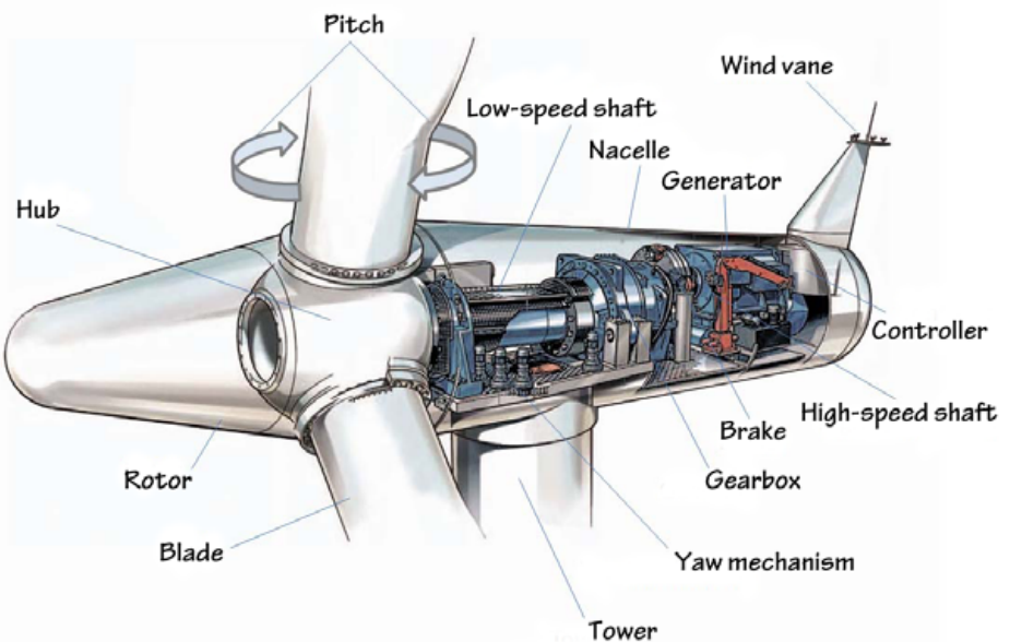
Diagram 2. The major components of a wind turbine
