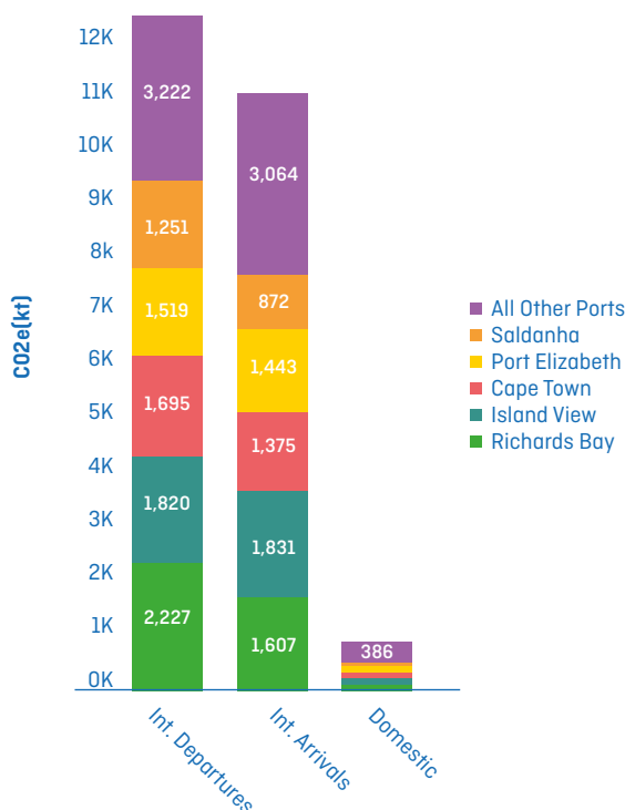
Figure 9: Maritime GHG emissions produced from South Africa’s ports international departures and arrivals in 2018.
