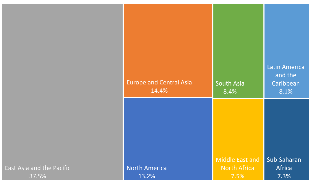
Figure 2.1. Regional shares of total GHG emissions, 2019
